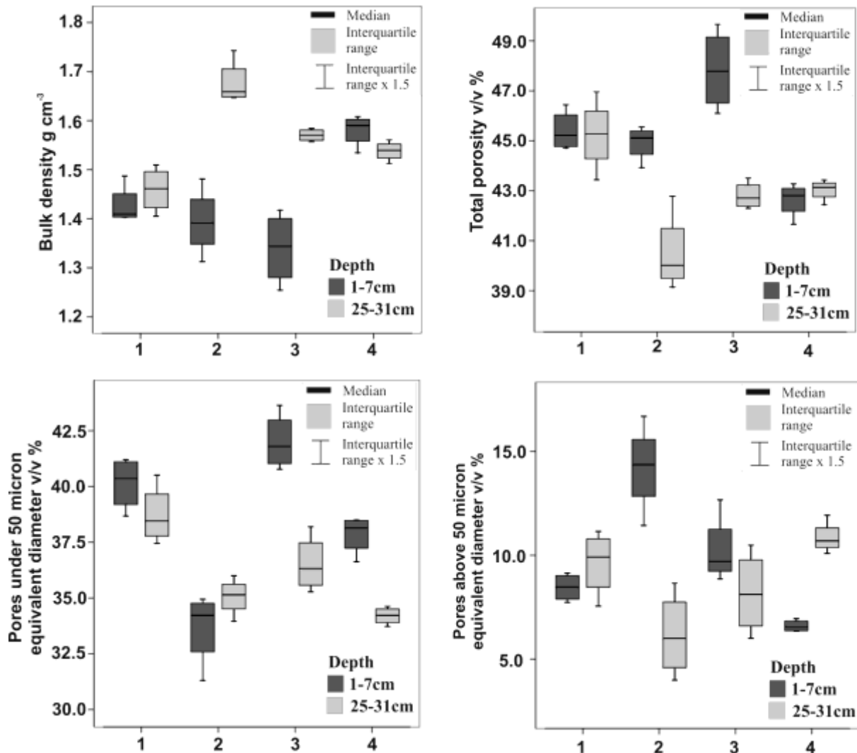
Figure 2. Porosity and bulk density conditions after different cultivation phases at two depths (in cm) of the study site (1: after chiseling (autumn), 2: after plowing, 3: seedbed conditions, after disking; 4: stubble field (late summer)).
