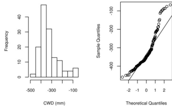
Figure 2. Histogram (left) and normal q-q plot (right) of asymmetric distribution of CWD
